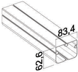
BIG CROSSBAR PROFILE
