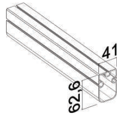
SMALL CROSSBAR PROFILE
