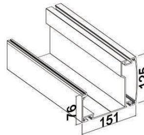
GUTTER
