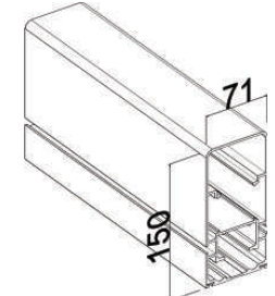
THIN RAIL
